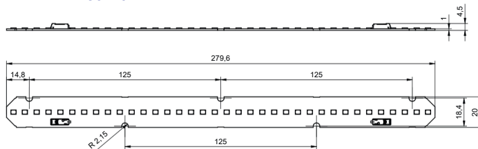
LinLED 280x20mm
