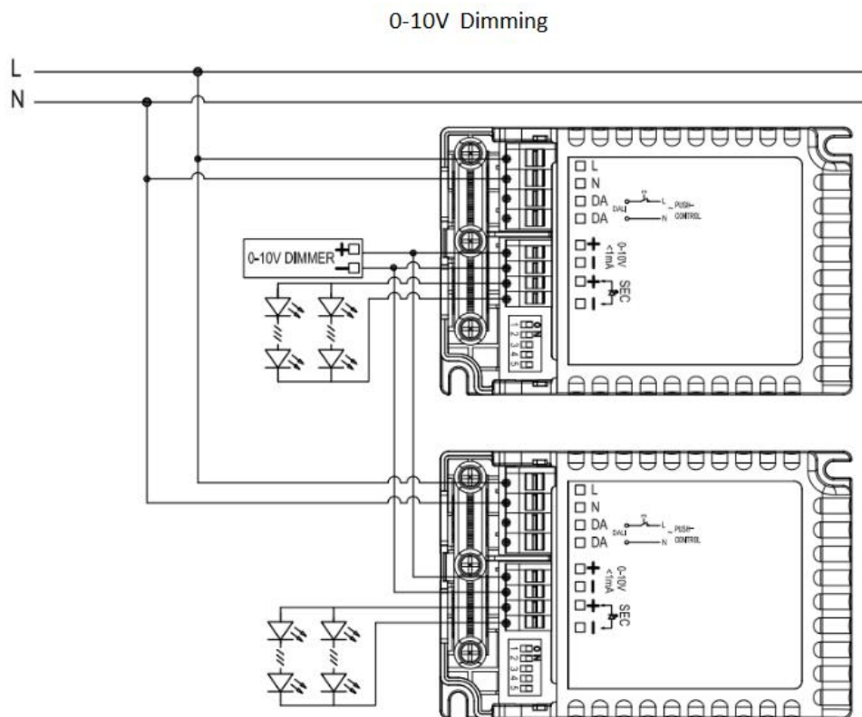
Fig. B: 0-10V Dimming
