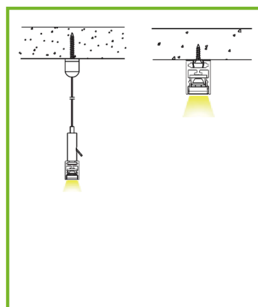
Installation
