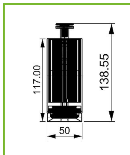
Dimensions with the front ring
